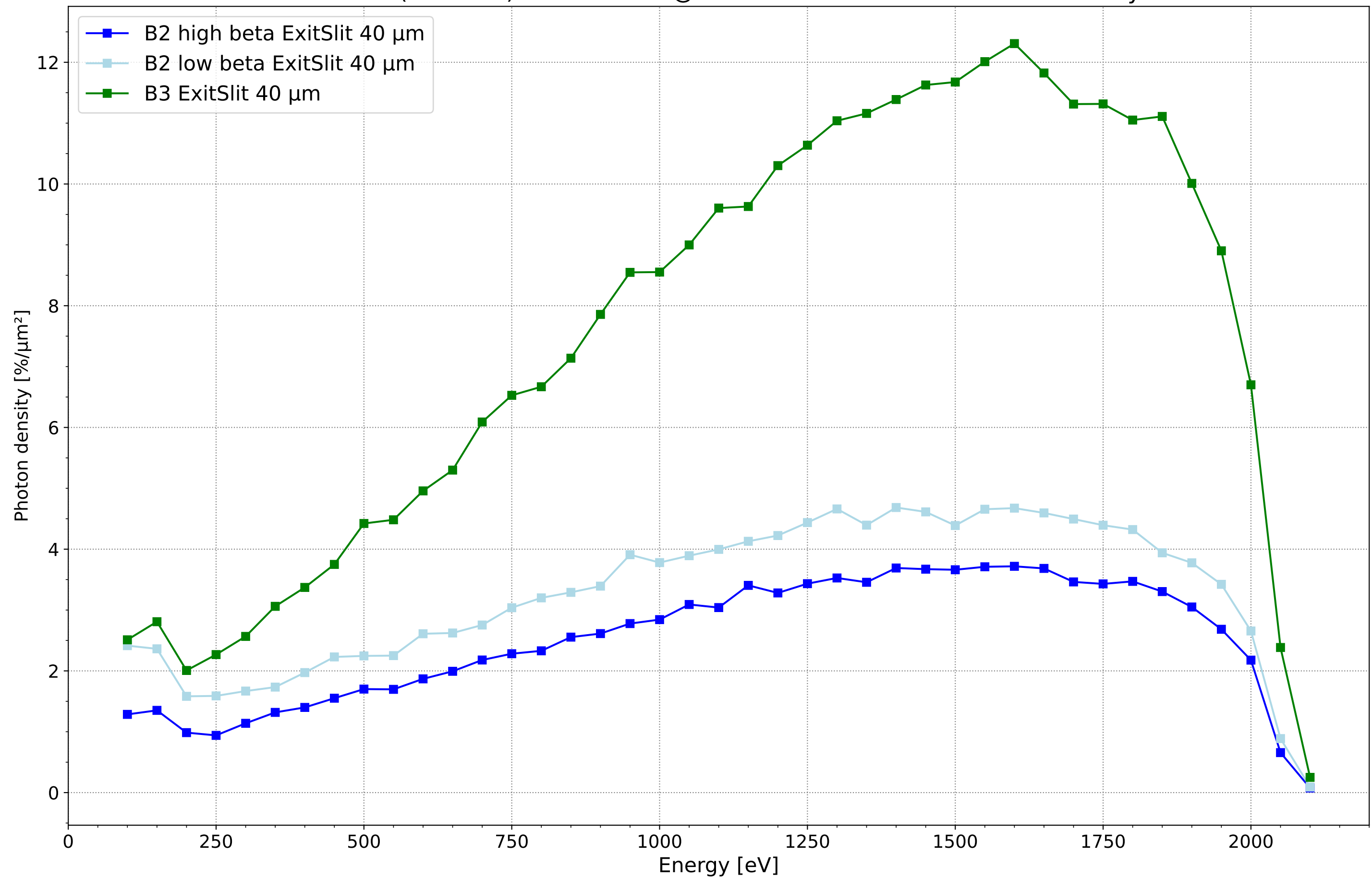
BESSY II (LowBeta) vs. BESSY III @ 56 m standard PGM-BL PhotonDensity
